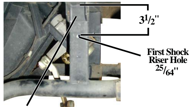
Shock Mount
